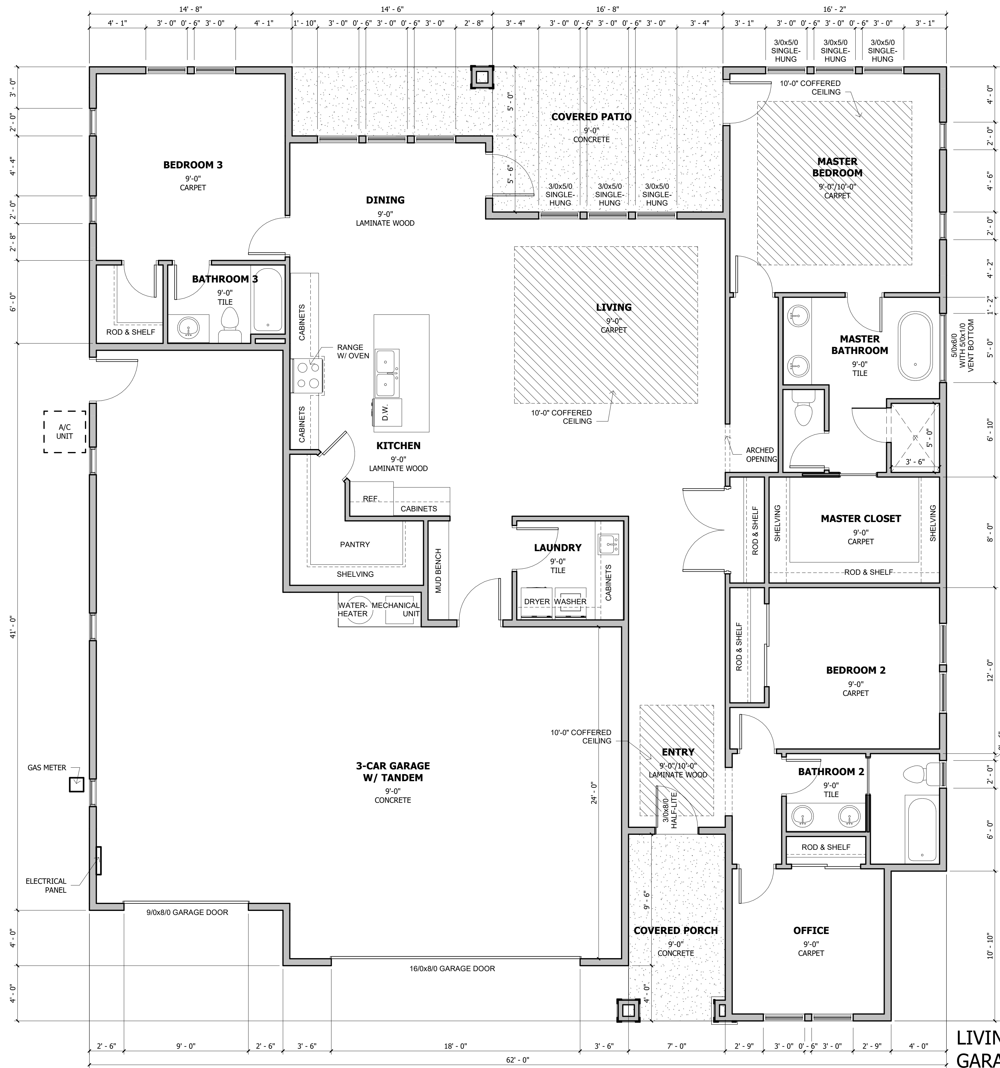
1 FLOOR PLAN 1/4" = 1'-0"
